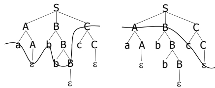
最左導出 (leftmost derivation)
